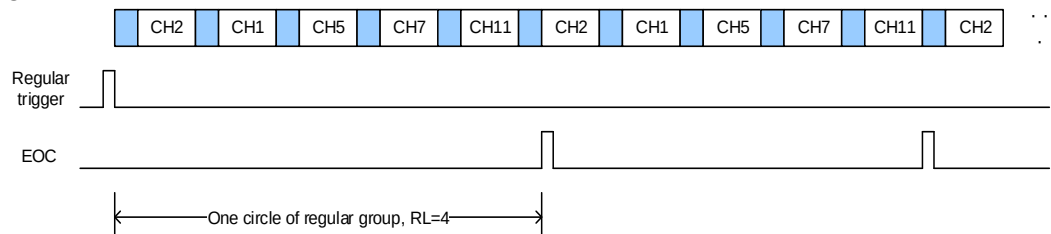
Figure 11-5. Scan conversion mode, continuous enable
