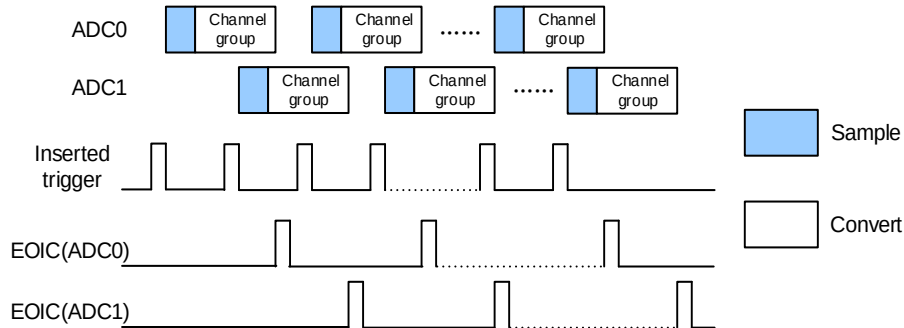
Figure 11-15. Trigger rotation: inserted channel group
