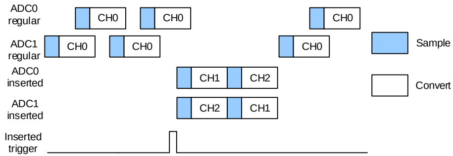
Figure 11-19 Follow-up single channel with inserted sequence CH1, CH2
