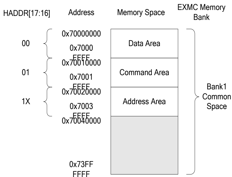
Figure 20-5. Diagram of bank1 common space
