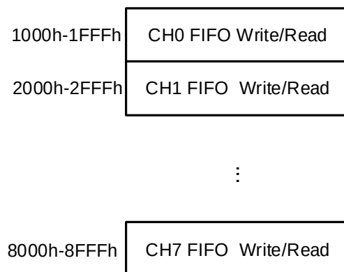
Figure 24-6. Host mode FIFO access register map
