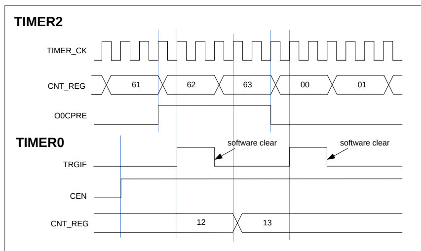
Figure 15-30. Pause TIMER0 with O0CPREF signal of Timer2
