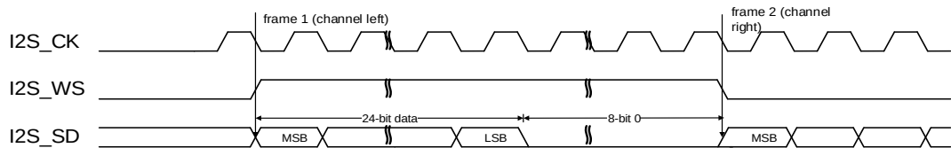
Figure 18-20. MSB justified standard timing diagram (DTLEN=01, CHLEN=1, CKPL=0)
