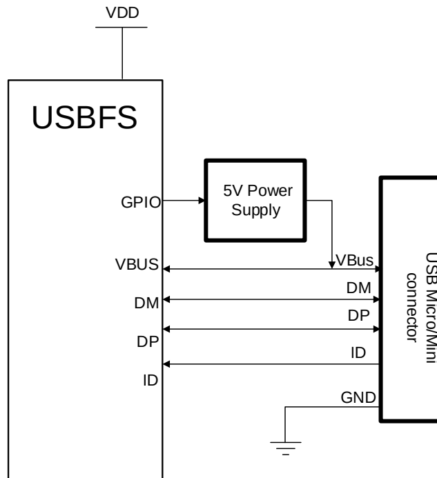
Figure 24-3. Connection with OTG mode
