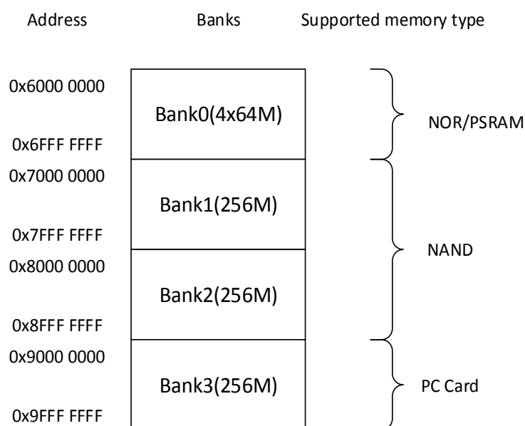
Figure 20-2. EXMC memory banks
