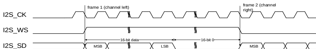
Figure 18-22. MSB justified standard timing diagram (DTLEN=00, CHLEN=1, CKPL=0)
