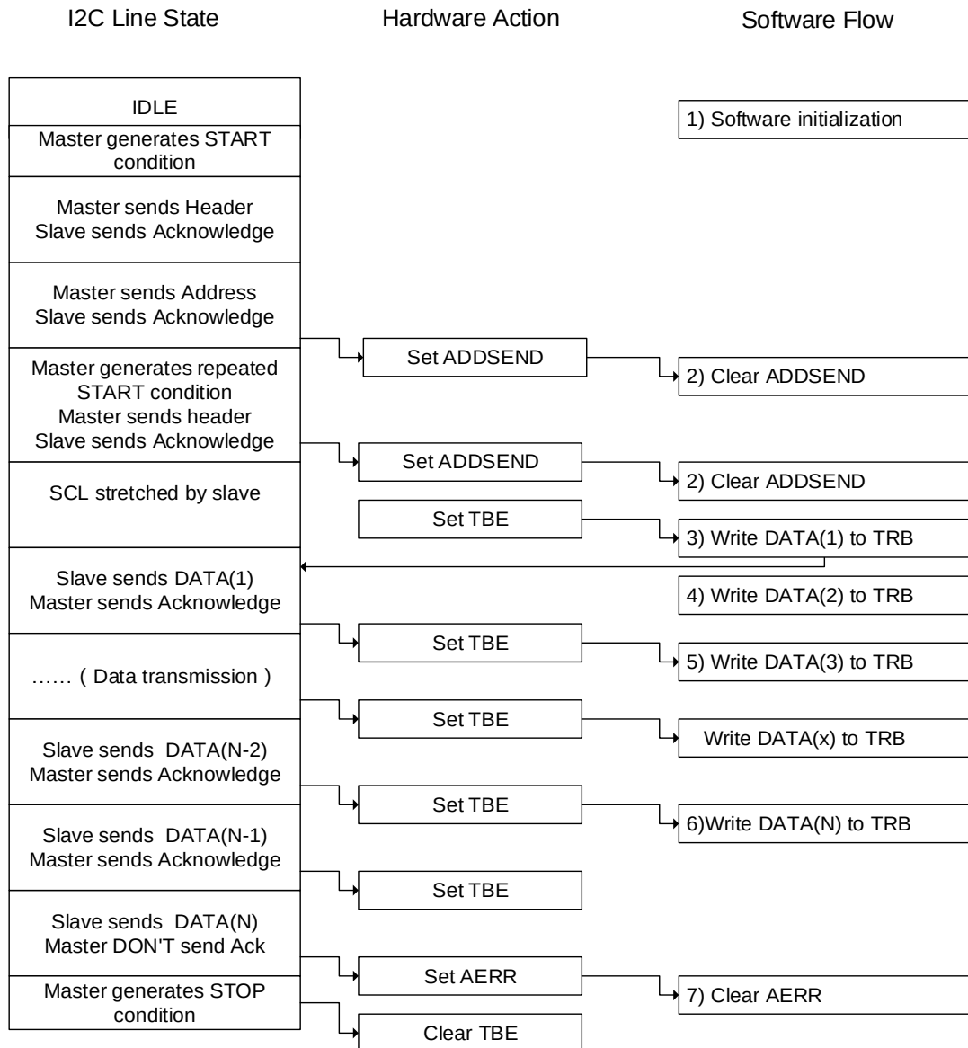
Figure 17-9. Programming model for slave transmitting
