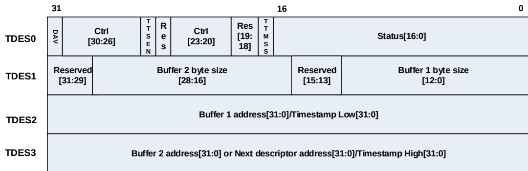
Figure 22-9. Transmit descriptor
