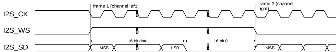
Figure 18-23. MSB justified standard timing diagram (DTLEN=00, CHLEN=1, CKPL=1)
