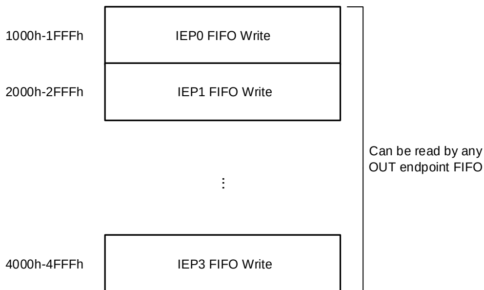
Figure 24-8. Device mode FIFO access register map
