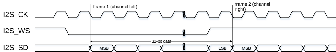
Figure 18-10. I2S Phillips standard timing diagram (DTLEN=10, CHLEN=1, CKPL=0)
