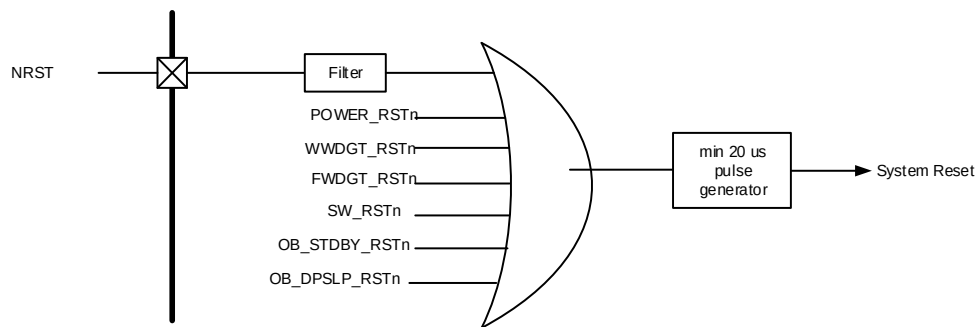
Figure 5-4. The system reset circuit
