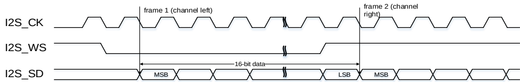
Figure 18-8. I2S Phillips standard timing diagram (DTLEN=00, CHLEN=0, CKPL=0)
