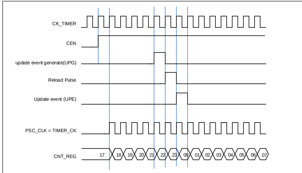
Figure 15-77. Normal mode, internal clock divided by 1
