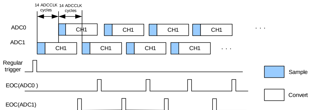
Figure 11-14. Follow-up slow mode on 1 channel
