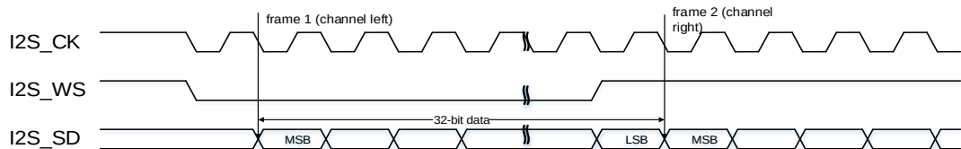
Figure 18-11. I2S Phillips standard timing diagram (DTLEN=10, CHLEN=1, CKPL=1)
