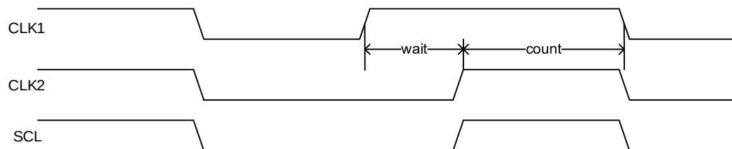
Figure 17-4. Clock synchronization
