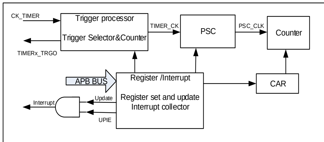
Figure 15-76. Basic timer block diagram
