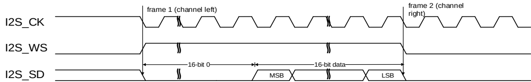
Figure 18-27. LSB justified standard timing diagram (DTLEN=00, CHLEN=1, CKPL=1)
