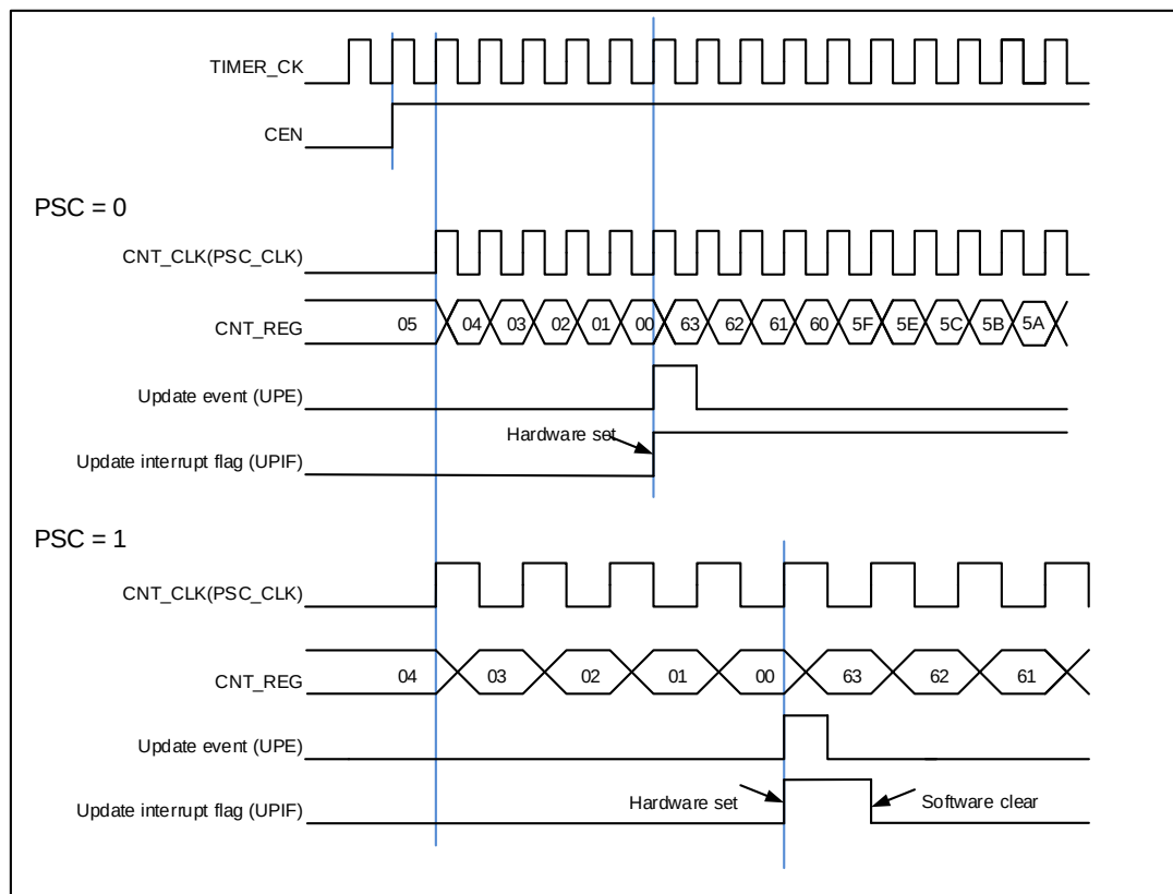
Figure 15-55. Down-counter timechart, PSC=0/1
