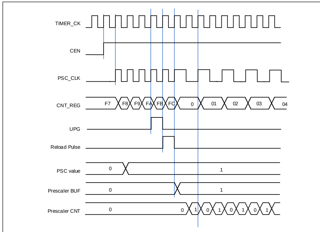
Figure 15-78. Counter timing diagram with prescaler division change from 1 to 2
