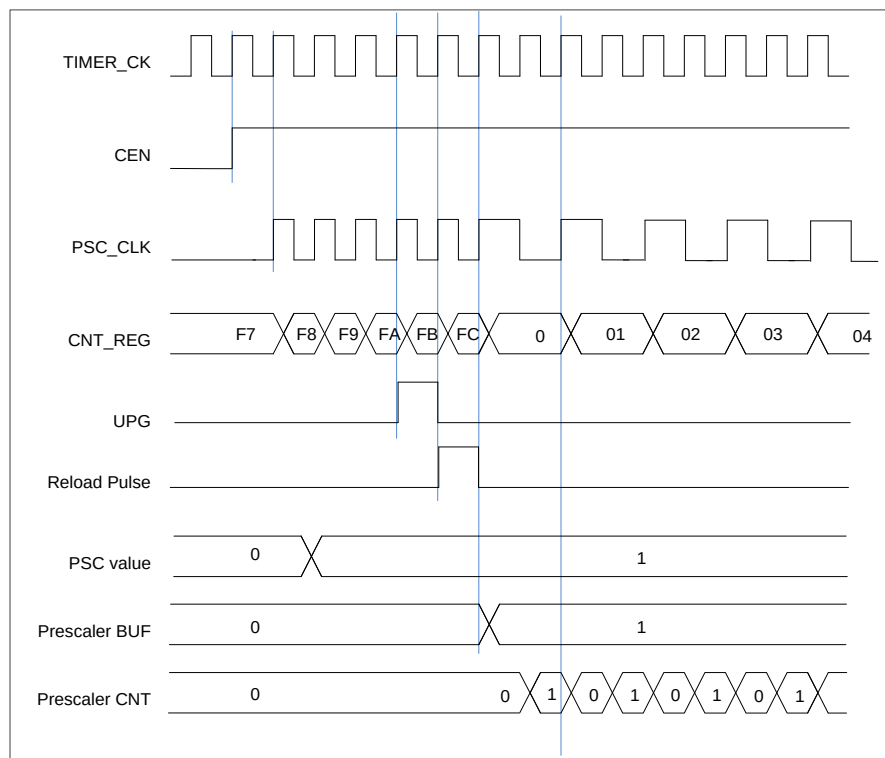
Figure 15-34. Counter timing diagram with prescaler division change from 1 to 2
