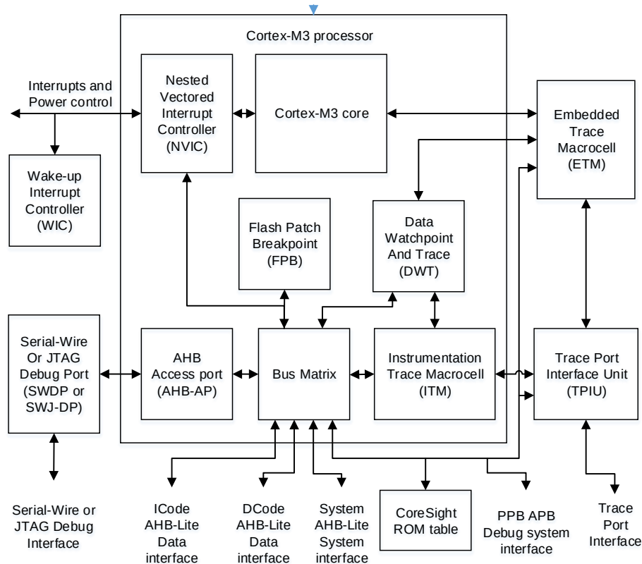
Figure 1-1. The structure of the Cortex™-M3 processor
