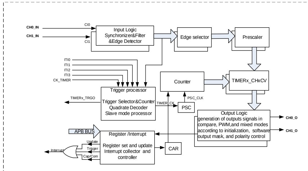
Figure 15-50. General level1 timer block diagram
