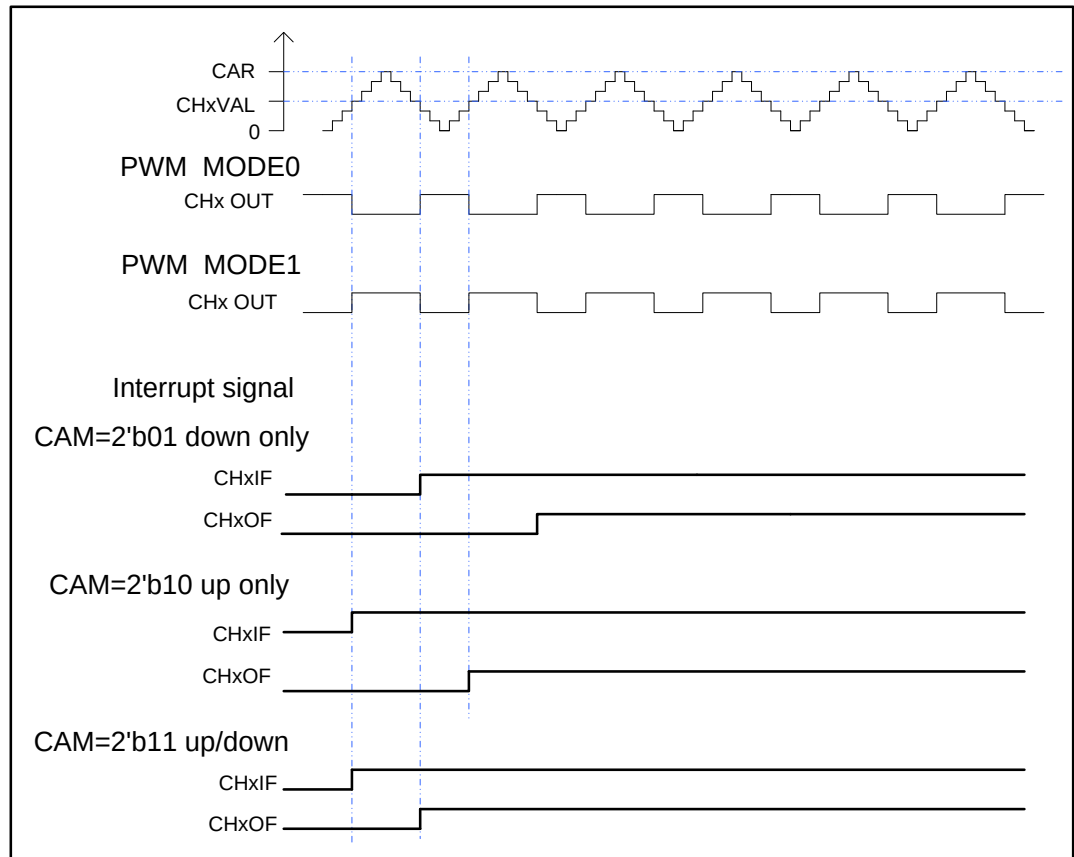
Figure 15-61. CAPWM timechart
