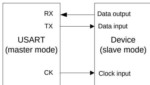
Figure 16-11. Example of USART in synchronous mode
