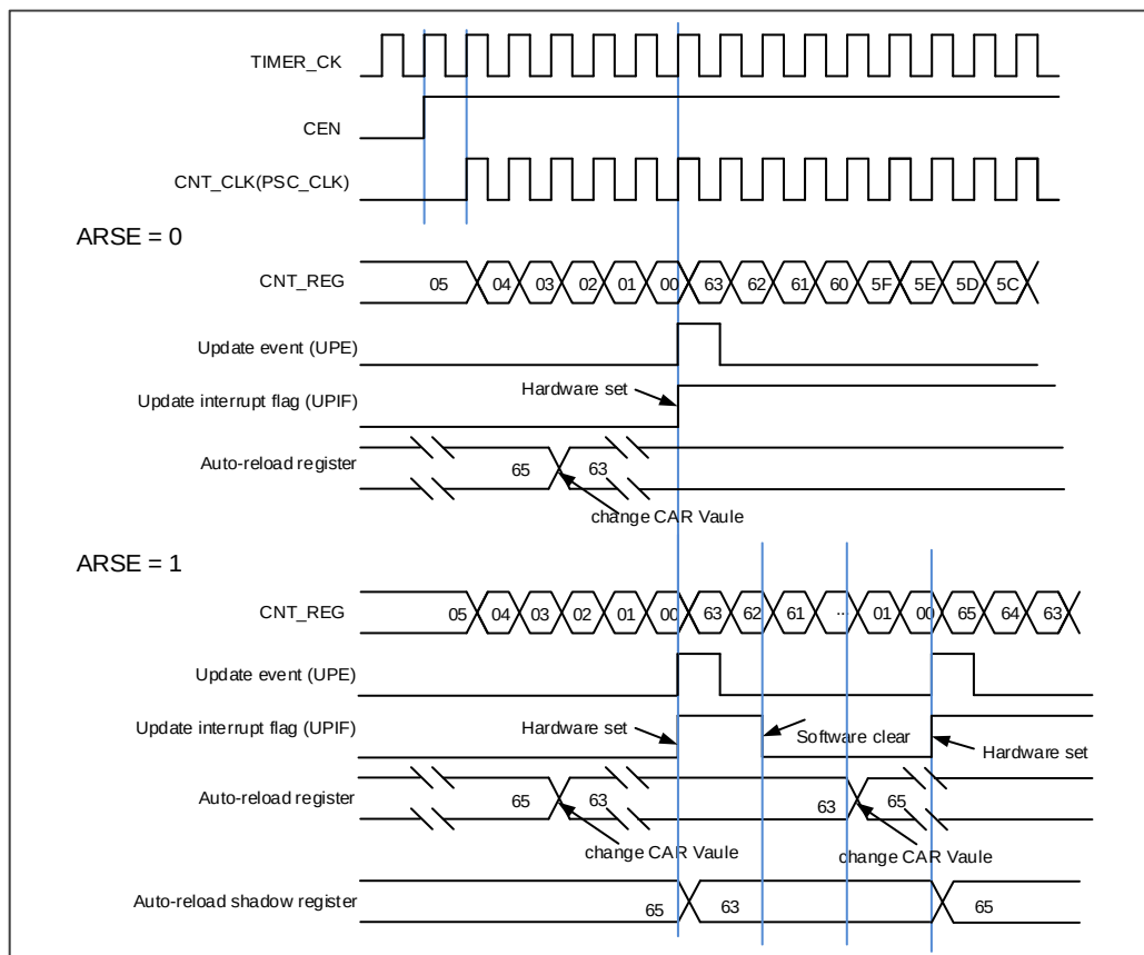
Figure 15-38. Down-counter timechart, change TIMEx_CAR on the go.
