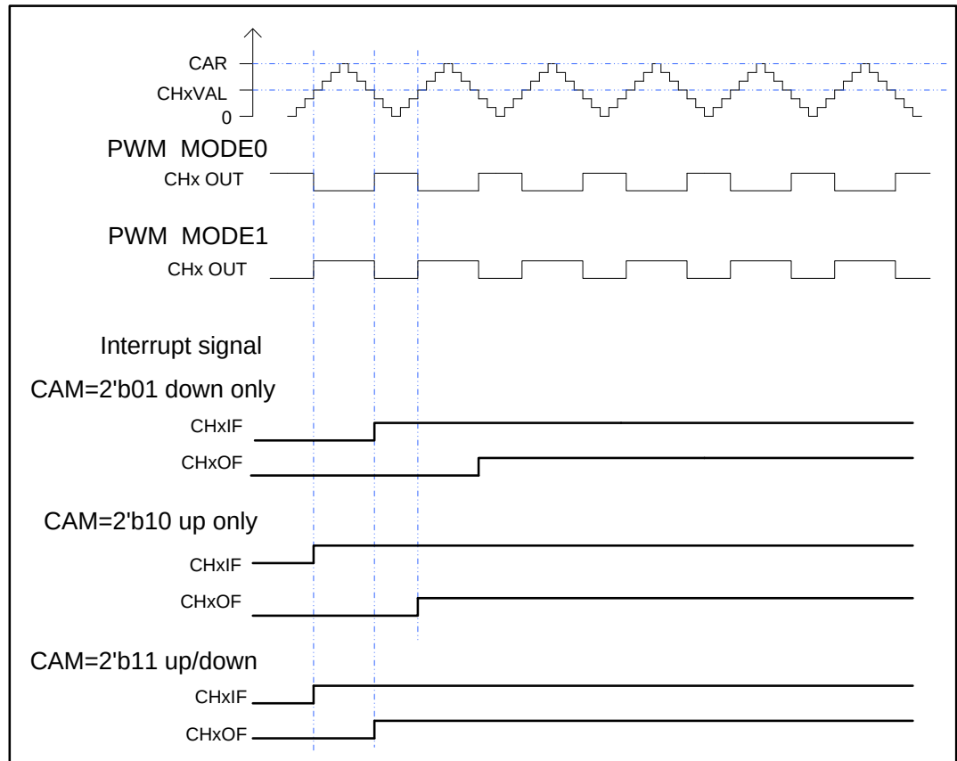
Figure 15-15. CAPWM timechart
