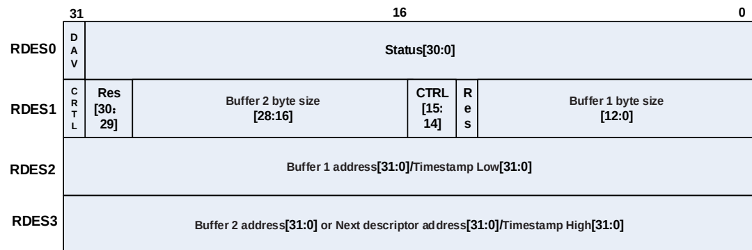
Figure 22-10. Receive descriptor
