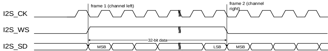
Figure 18-18. MSB justified standard timing diagram (DTLEN=10, CHLEN=1, CKPL=0)
