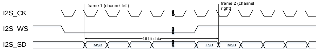
Figure 18-9. I2S Phillips standard timing diagram (DTLEN=00, CHLEN=0, CKPL=1)
