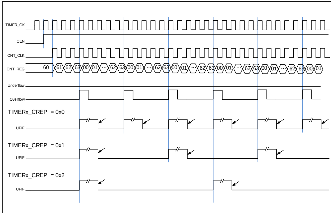
Figure 15-10. Repetition timechart for up-counter
