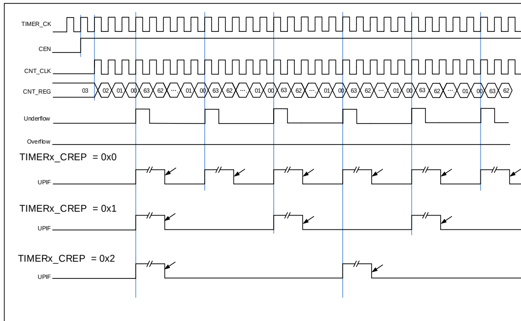
Figure 15-11. Repetition timechart for down-counter
