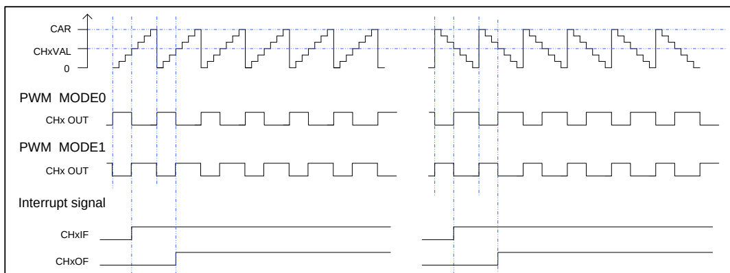
Figure 15-42. EAPWM timechart
