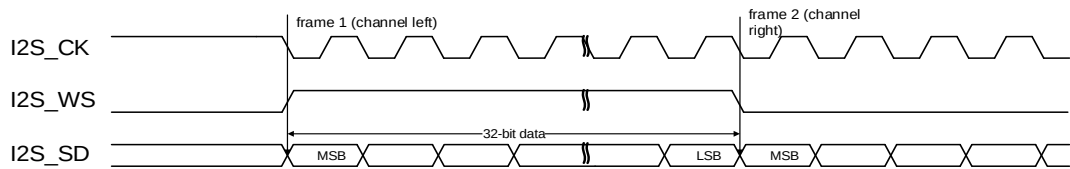
Figure 18-19. MSB justified standard timing diagram (DTLEN=10, CHLEN=1, CKPL=1)
