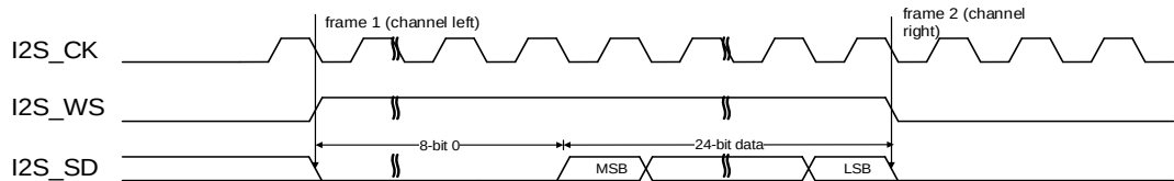
Figure 18-24. LSB justified standard timing diagram (DTLEN=01, CHLEN=1, CKPL=0)
