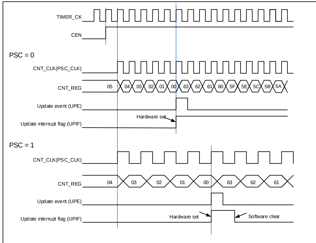
Figure 15-71. Down-counter timechart, PSC=0/1
