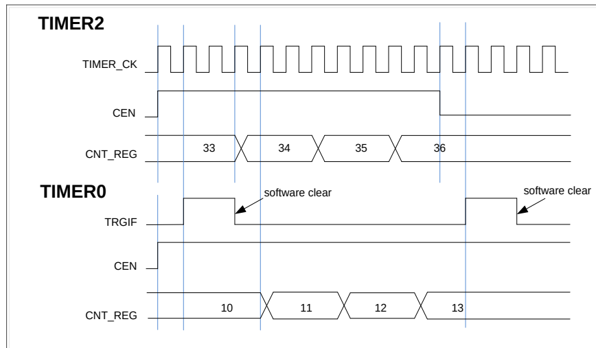
Figure 15-29. Pause TIMER0 with enable signal of TIMER2
