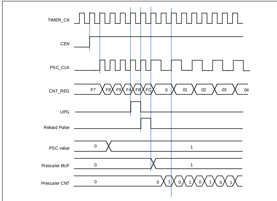
Figure 15-3. Counter timing diagram with prescaler division change from 1 to 2 (PSC value change from 0 to 1)
