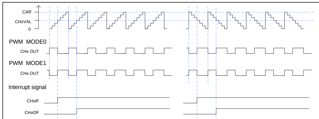
Figure 15-14. EAPWM timechart
