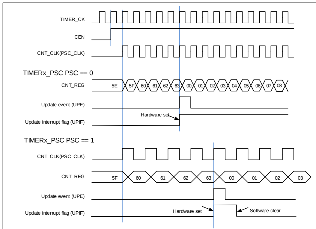
Figure 15-69. Up-counter timechart, PSC=0/1
