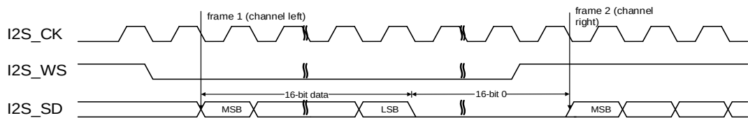
Figure 18-14. I2S Phillips standard timing diagram (DTLEN=00, CHLEN=1, CKPL=0)
