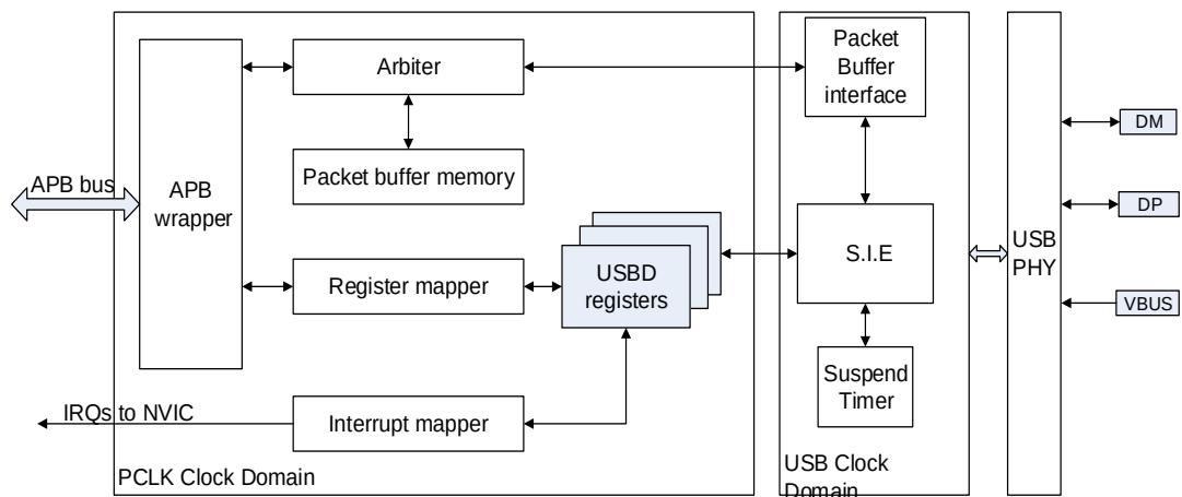
Figure 23-1. USBD block diagram
