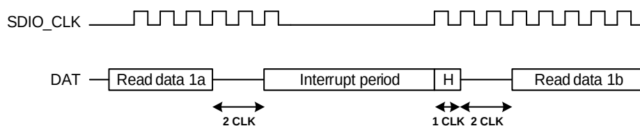
Figure 19-12. Read wait control by stopping SDIO_CLK
