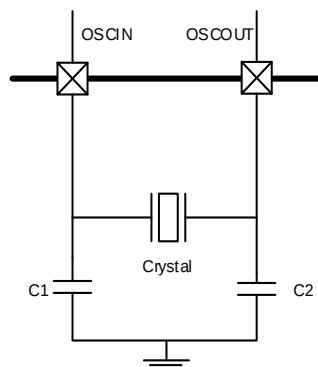
Figure 5-6. HXTAL clock source
