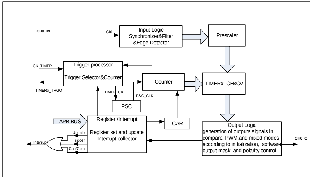
Figure 15-66. General level2 timer block diagram
