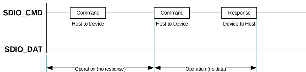
Figure 19-1. SDIO “no response” and “no data” operations
