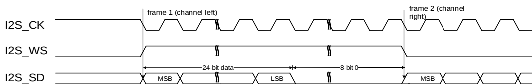
Figure 18-21. MSB justified standard timing diagram (DTLEN=01, CHLEN=1, CKPL=1)
