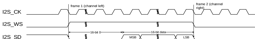
Figure 18-26. LSB justified standard timing diagram (DTLEN=00, CHLEN=1, CKPL=0)
