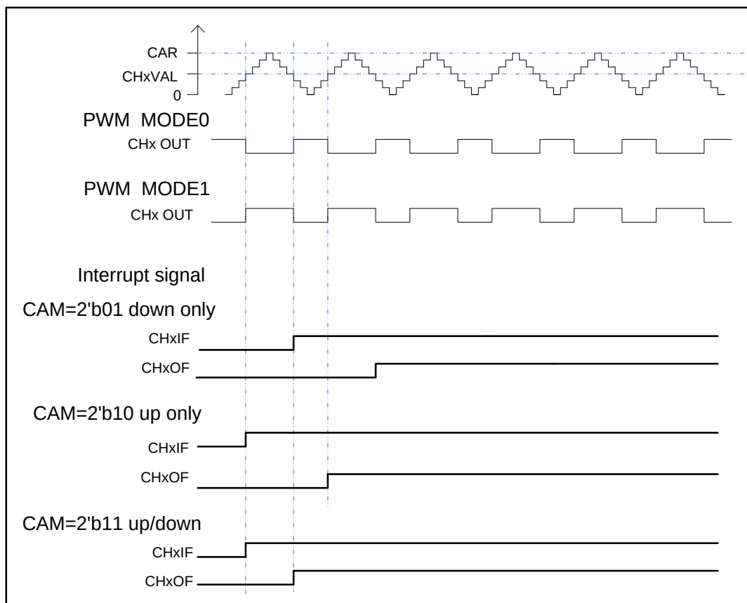
Figure 15-43. CAPWM timechart
