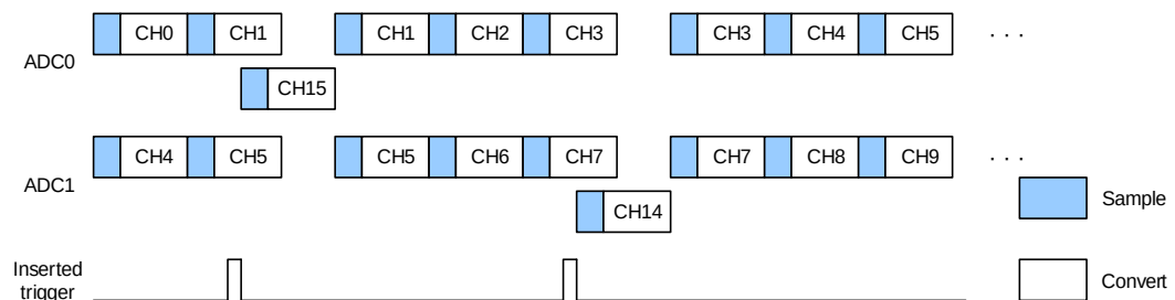
Figure 11-17. Regular parallel & trigger rotation mode
