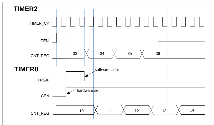
Figure 15-27. Triggering TIMER0 with enable signal of TIMER2
