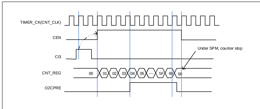
Figure 15-65. Single pulse mode TIMERx\_CHxCV = 0x04 TIMERx\_CAR=0x60
