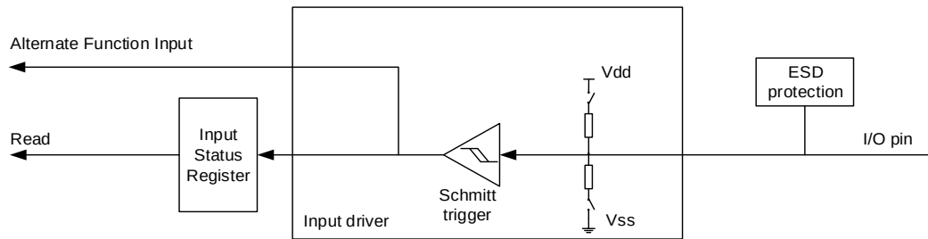
Figure 7-2. Input configuration
