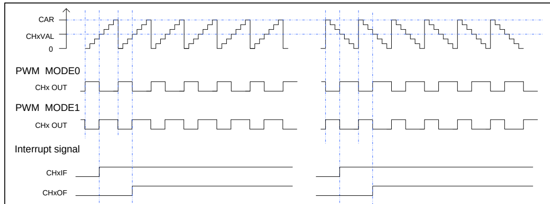
Figure 15-60. EAPWM timechart
