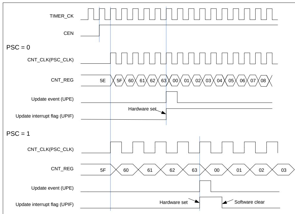
Figure 15-35. Up-counter timechart, PSC=0/1
