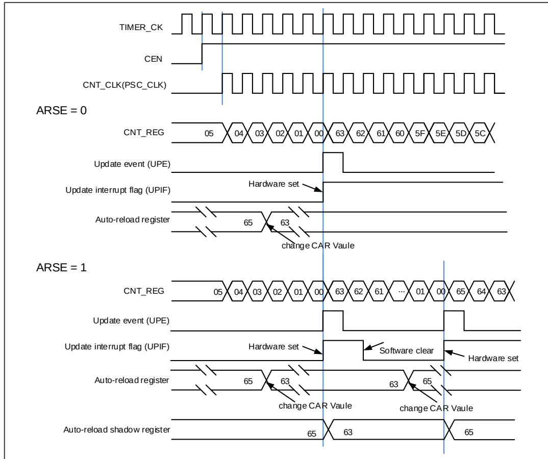
Figure 15-56. Down-counter timechart, change TIMERx_CAR on the go
