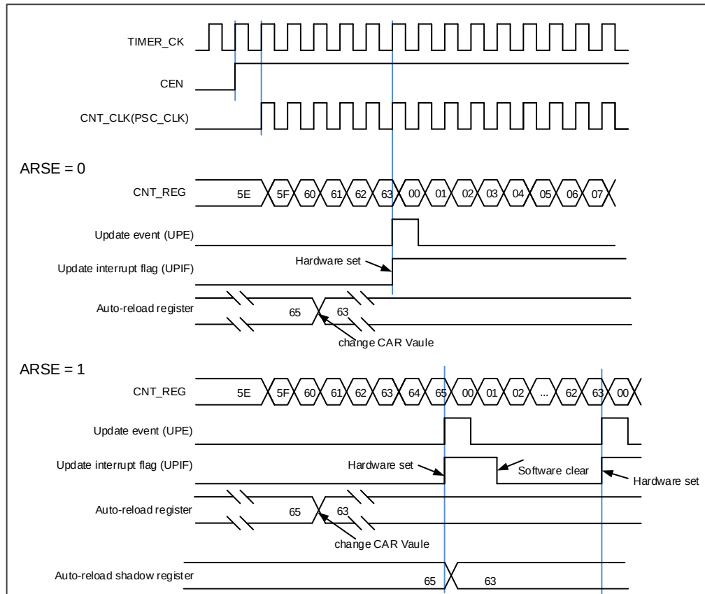
Figure 15-80. Up-counter timechart, change TIMERx_CAR on the go
