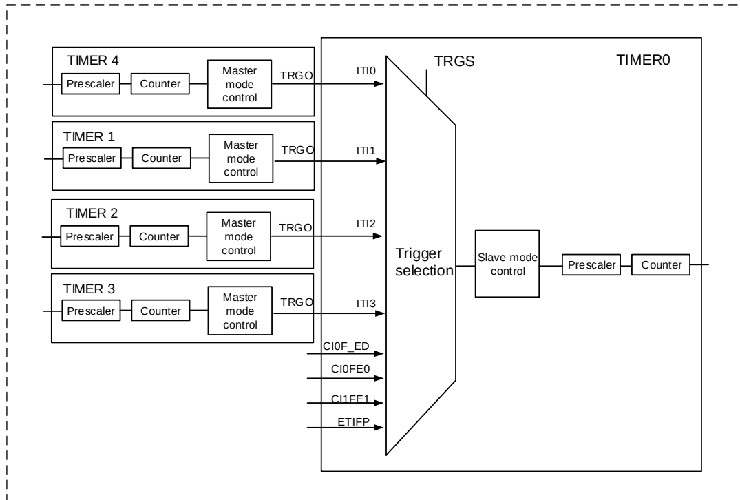
Figure 15-26. Timer0 master/slave mode timer example
