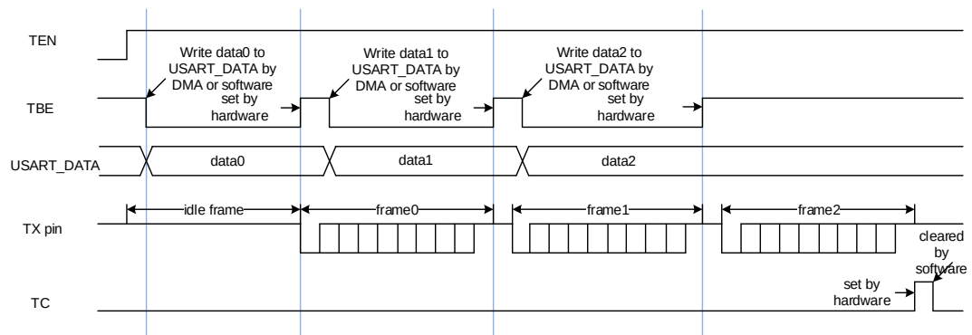
Figure 16-3. USART transmit procedure
