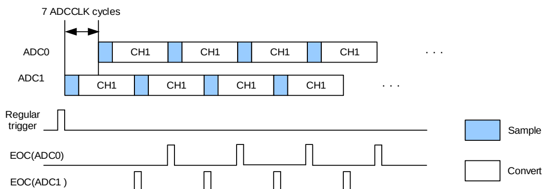
Figure 11-13. Follow-up fast mode on 1 channel in continuous conversion mode
