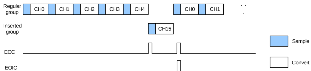
Figure 11-7. Auto-insertion, CTN = 1
