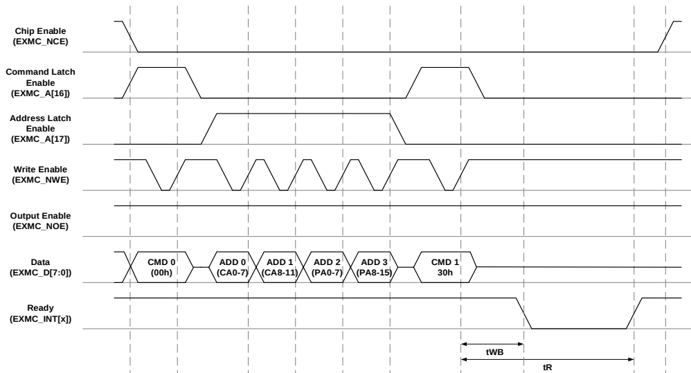
Figure 20-24. Access to none "NCE don't care" NAND Flash
