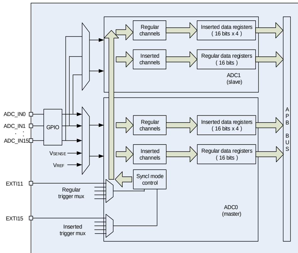
Figure 11-10. ADC sync block diagram
