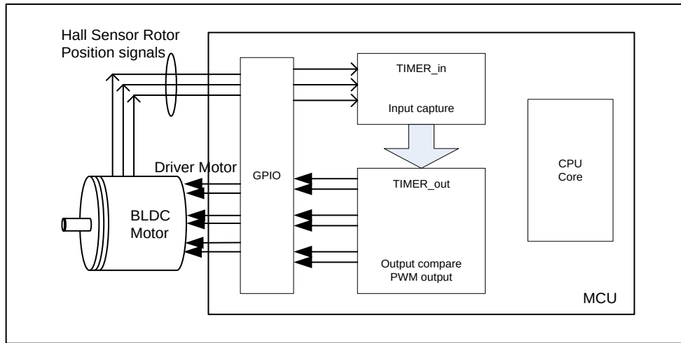
Figure 15-21. Hall sensor timing between two timers
