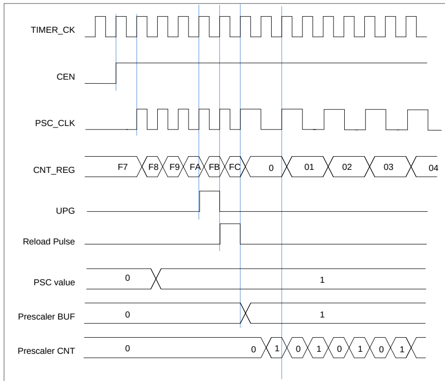
Figure 15-52. Counter timing diagram with prescaler division change from 1 to 2
