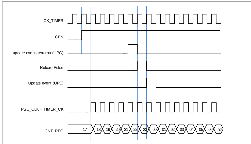
Figure 15-67. Normal mode, internal clock divided by 1
