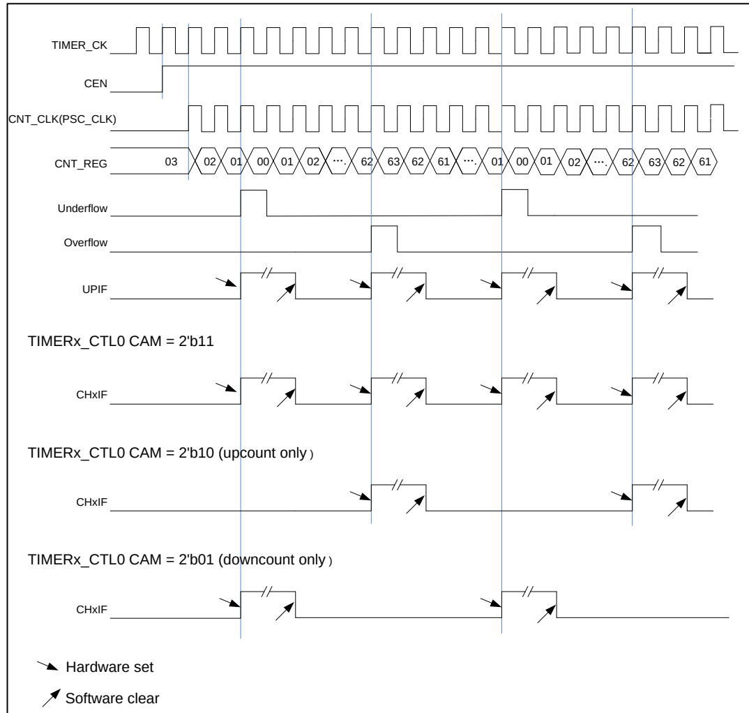
Figure 15-57. Center-aligned counter timechart
