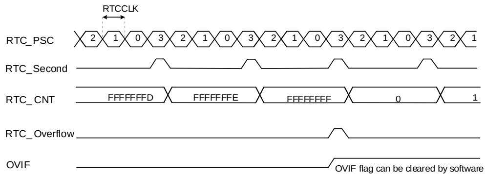
Figure 14-3. RTC second and overflow waveform example (RTC_PSC= 3)
