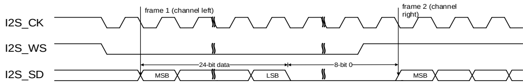
Figure 18-13. I2S Phillips standard timing diagram (DTLEN=01, CHLEN=1, CKPL=1)
