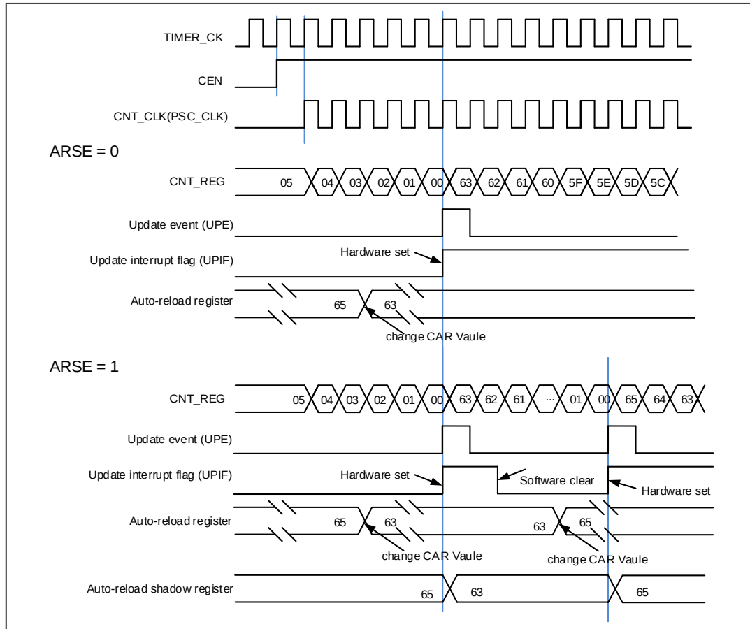
Figure 15-72. Down-counter timechart, change TIMERx_CAR on the go
