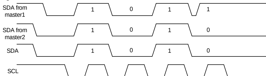
Figure 17-5. SDA Line arbitration
