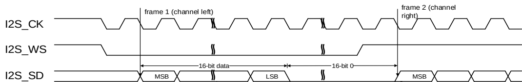
Figure 18-15. I2S Phillips standard timing diagram (DTLEN=00, CHLEN=1, CKPL=1)
