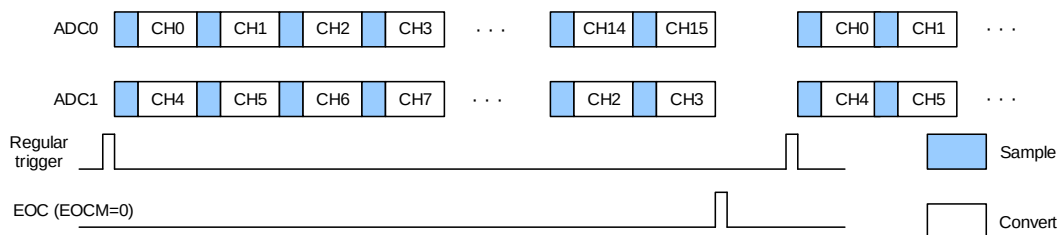
Figure 11-11. Regular parallel mode on 16 channels
