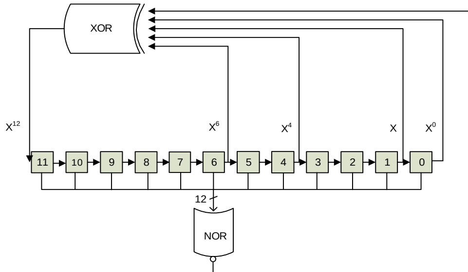
Figure 12-2. DAC LFSR algorithm
