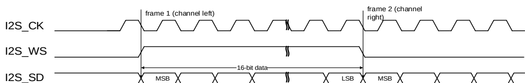
Figure 18-16. MSB justified standard timing diagram (DTLEN=00, CHLEN=0, CKPL=0)
