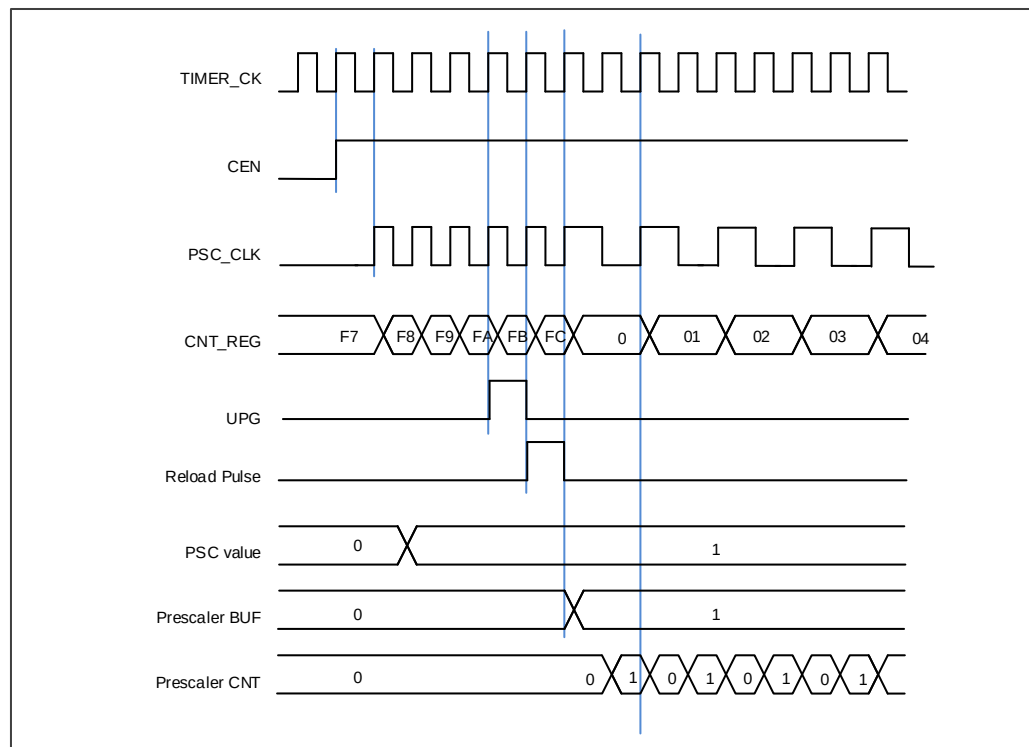
Figure 15-68. Counter timing diagram with prescaler division change from 1 to 2
