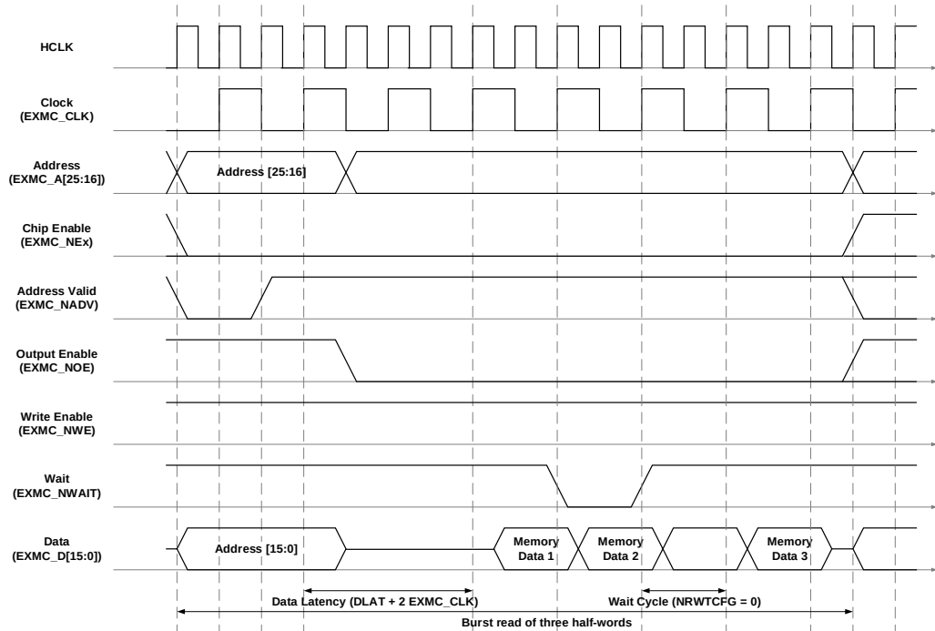
Figure 20-21. Synchronous mux burst read timing
