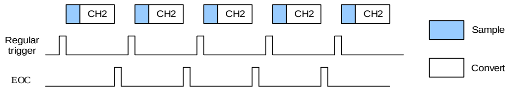
Figure 11-2. Single conversion mode
