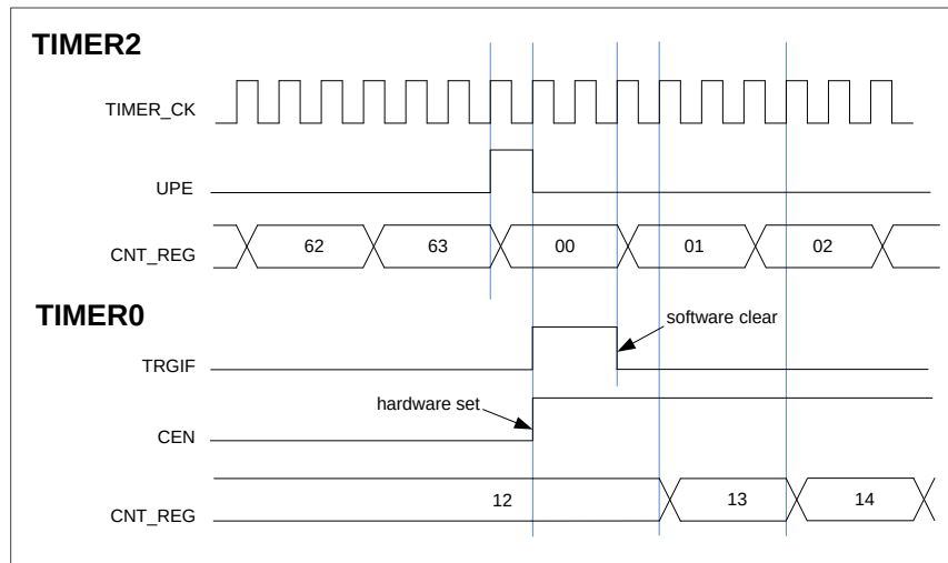
Figure 15-28. Triggering TIMER0 with update signal of TIMER2
