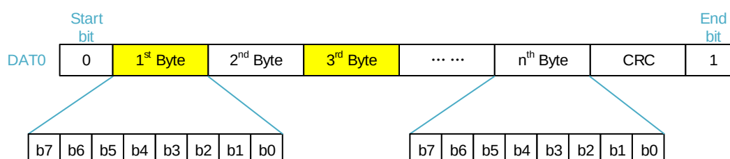
Figure 19-9. 1-bit data bus width
