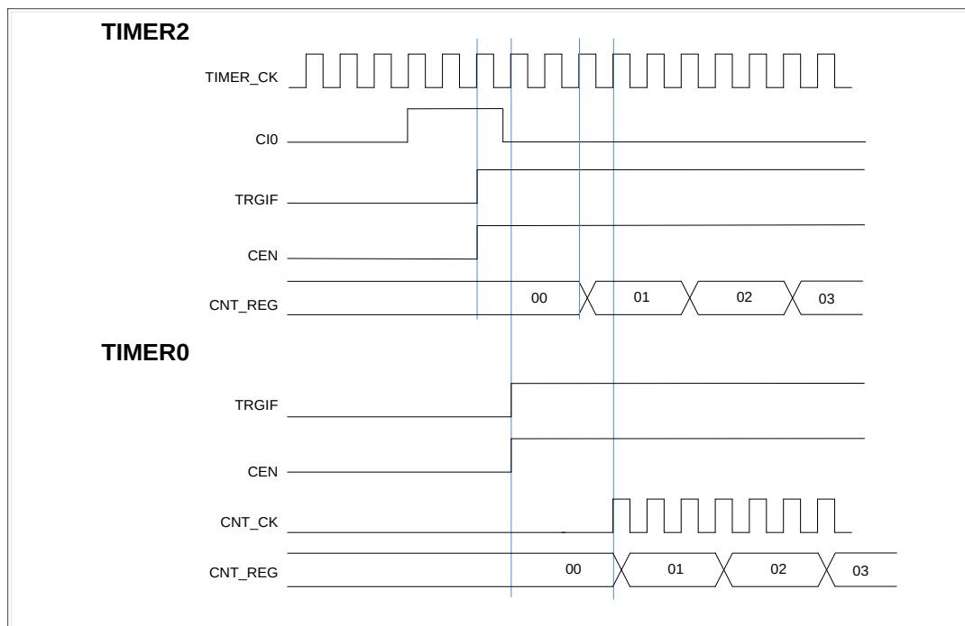
Figure 15-31. Triggering TIMER0 and TIMER2 with TIMER2's CI0 input
