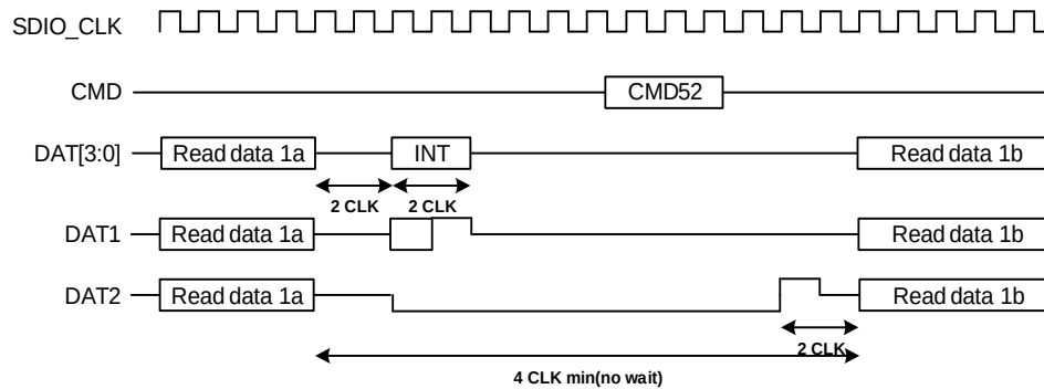
Figure 19-13. Read wait operation using SDIO_DAT[2]
