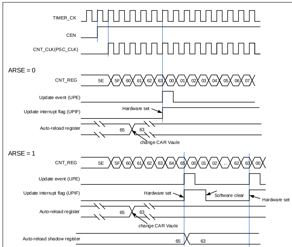
Figure 15-70. Up-counter timechart, change TIMERx_CAR on the go
