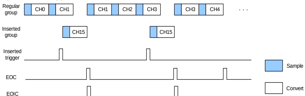
Figure 11-8. Triggered insertion
