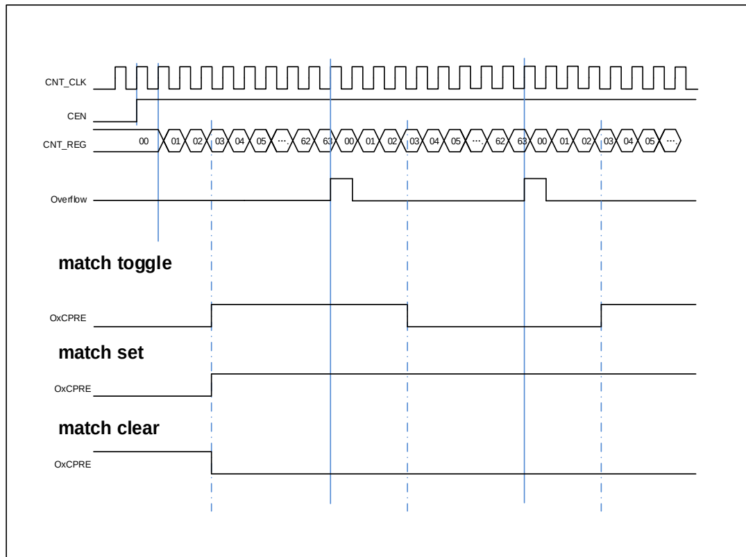
Figure 15-59. Output-compare under three modes
